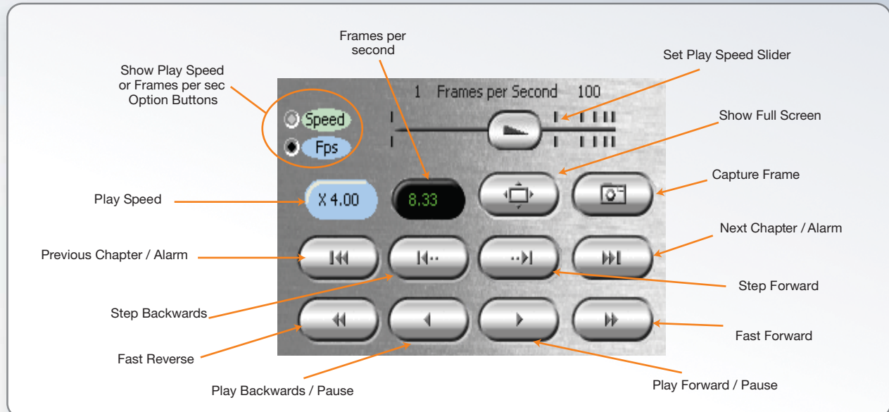
DVD-Explorer Replay Buttons & Controls
